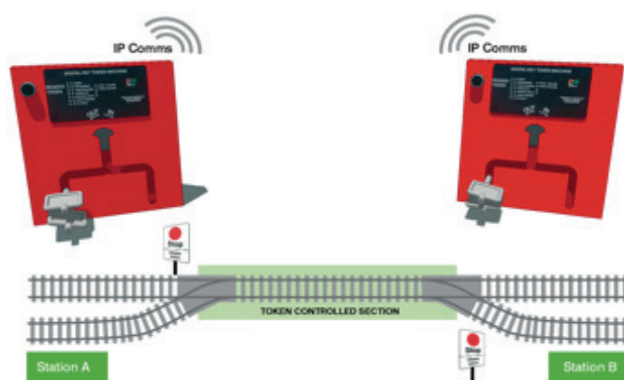
Figure 2: Example application on a single line section of railway
